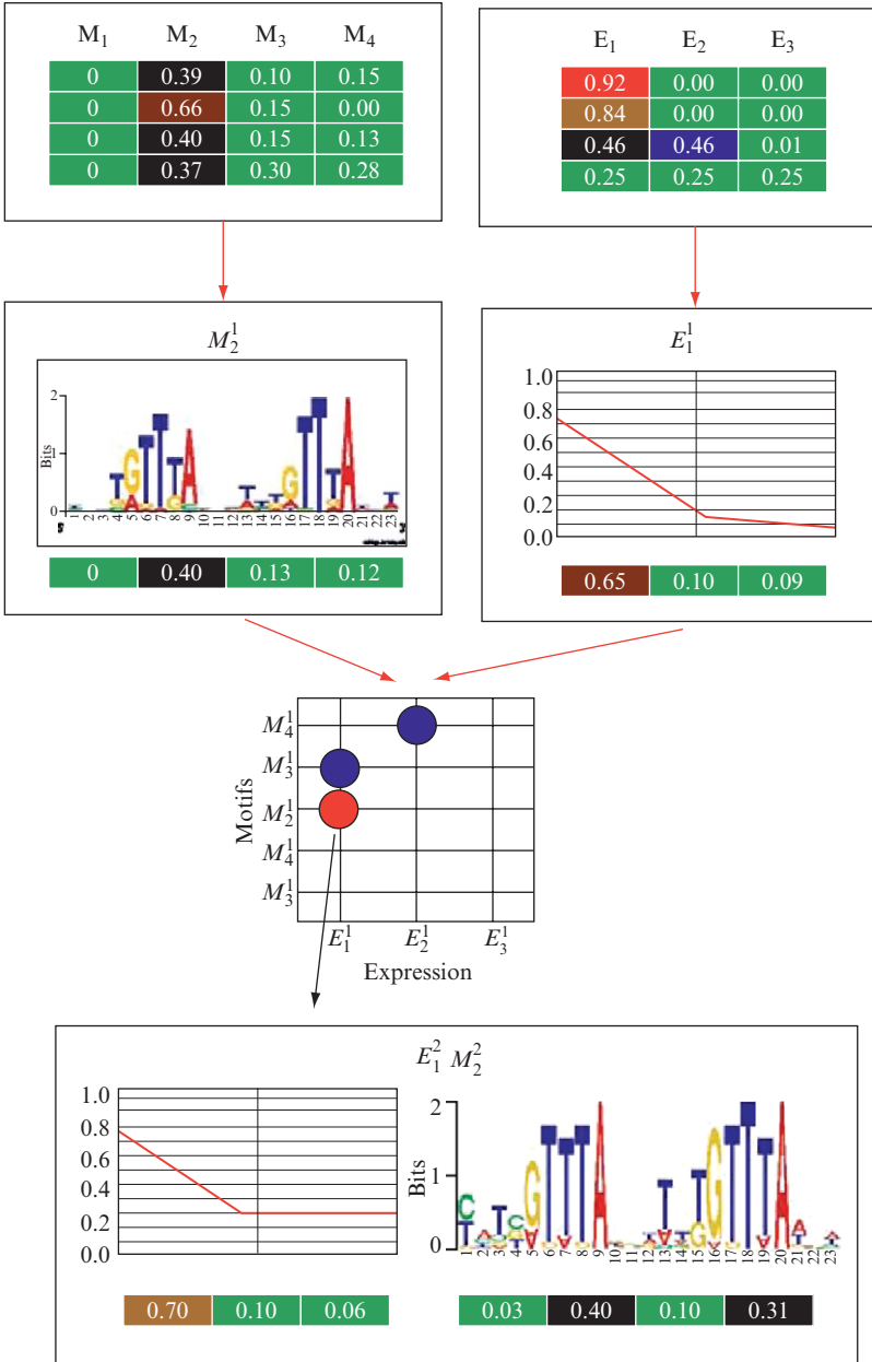
FIG. 4. Using GPS to build promoter profiles. GPS generation of the profile E_1^2 M_2^2 is shown here. It partially corresponds to the highlighted substructure of the lattice shown in Fig. 5. GPS starts by using information from databases and microarray data to construct a family of models
